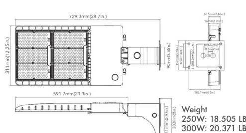
LARGE 250W & 300W Wall Mount
